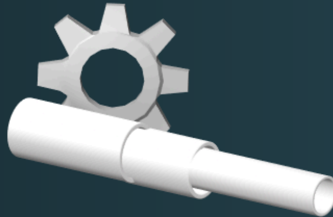
ETL Pipeline
